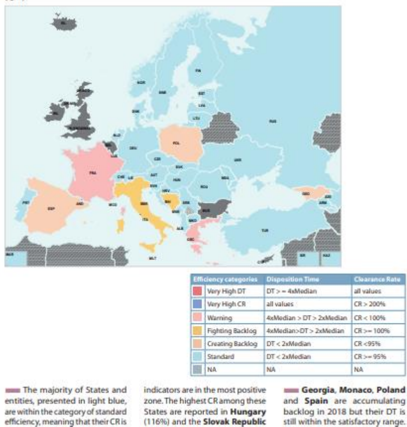
Map 5.8 Clearance Rate vs Disposition Time for civil and commercial litigious cases at first instance in 2018 (Q91)
